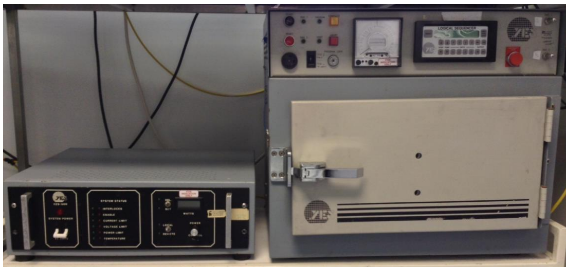
Figure. 3.8. YES-R3 oxygen plasma etching system.
