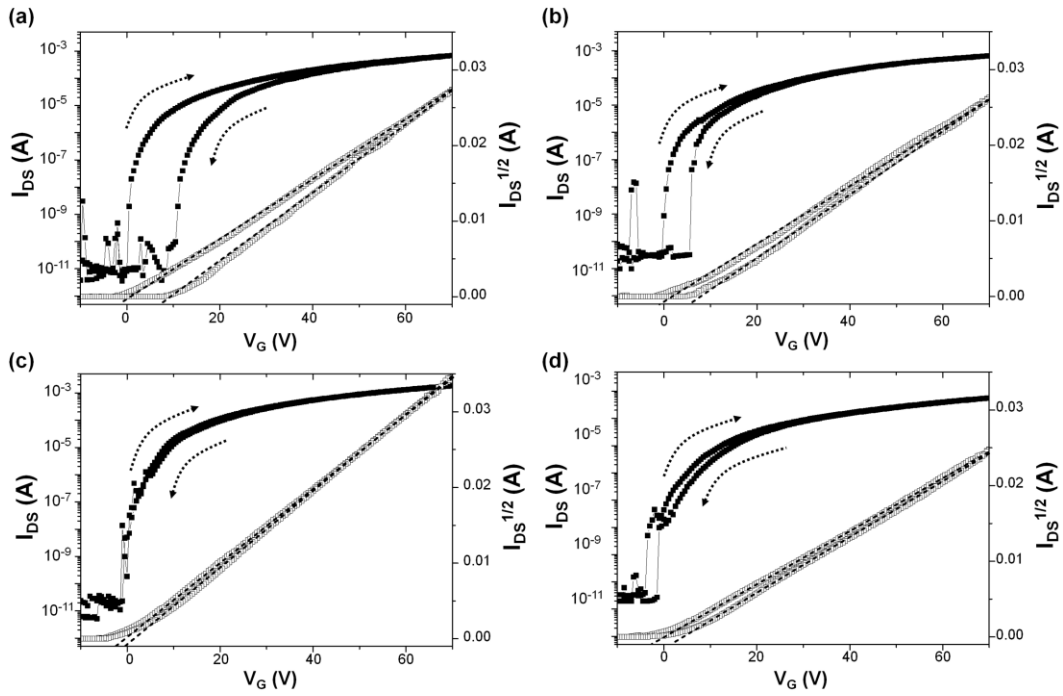
Figure. 6.2. Transfer characteristics ( I_{DS} vs V_G curve—full symbols) in the saturation region ( V_{DS}=50 V) of (a) reference, (b) 10 min, (c) 15 min, and (d) 30 min plasma treated ZnO TFTs. For each set of data, plots of (I_{DS})^{1/2} versus V_G are also shown (open symbols).
