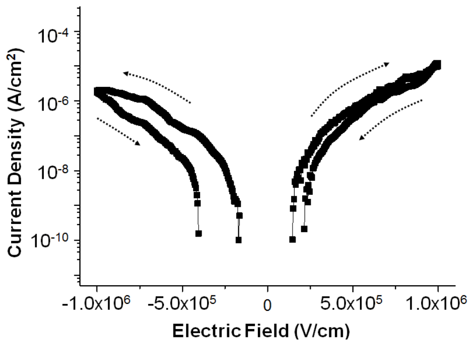
Figure. 7.7. Current density versus electric field for Al/CAPS/Al structure.
